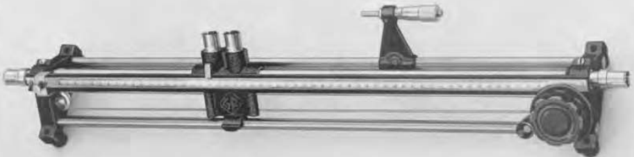
Figure 1. View of the Type 874-LBA Slotted Line with Type 874-LV Micrometer Vernier.
