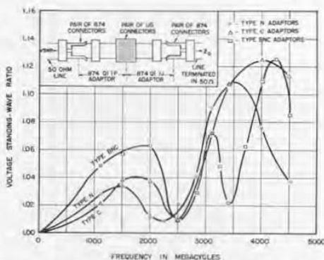
Figure 6. VSWR as a function of frequency for typical adaptors. Measurements were made on pairs of adaptor units, as shown in the sketch, and hence, the standing-wave ratios shown are the totals produced by two pairs of Type 874 Connectors plus a pair of UG-type (i.e., N, C, or BNC) connectors.
