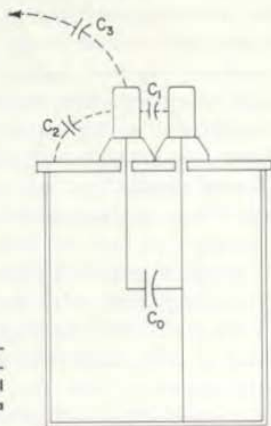
Figure 1. Schematic diagram showing the terminal capacitances of a capacitor.
