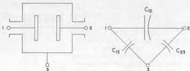
Figure 8. Diagram and schematic of 3-terminal capacitor.
