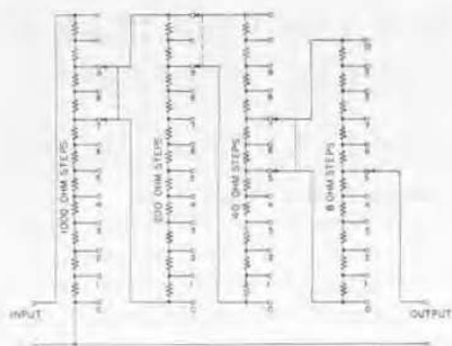
Figure 1. Schematic diagram of Type 1454 Decade Voltage Divider.
