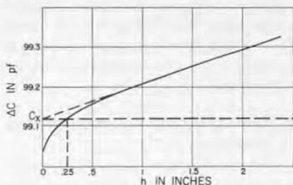
Figure 6. Determination of unknown capacitance C_x from \Delta C measured with fine-wire connector. At h = \frac{1}{4} inch C_x = \Delta C . (From Field paper 10 )
